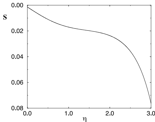
Figure 1. The RS entropy S at zero temperature as a function of the threshold \eta .
