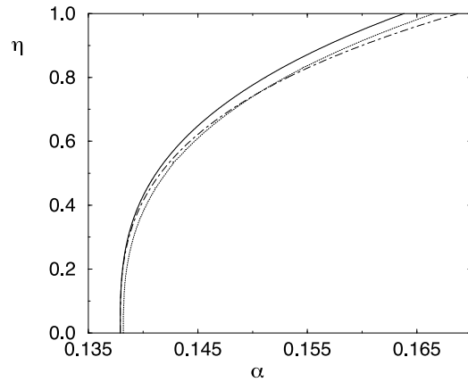
Figure 2. The critical capacity in the RS (full curve) and RSB1 (dotted curve) approximation as a function of the threshold \eta . For comparison we also show the results of [5] (dashed-dotted curve).
